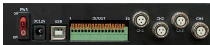
[Rear panel]
